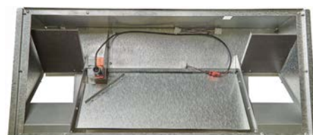
Commercial Room Ventilator-Fixed
